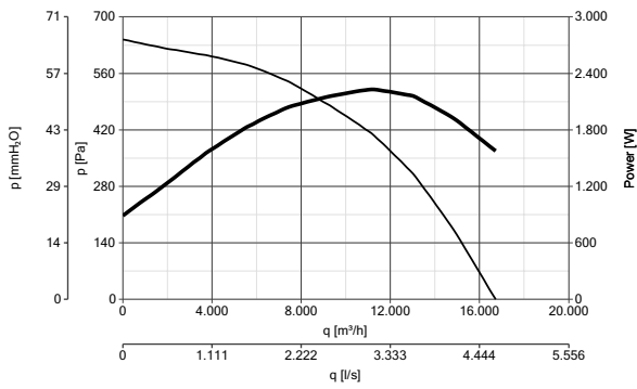
VORT QBK HE COMFORT 710 6T
