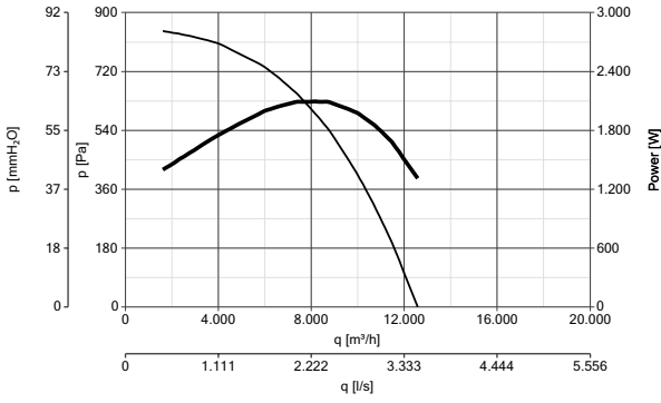
VORT QBK HE COMFORT 560 4T
